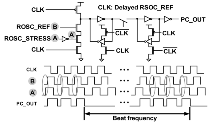
Fig. 5. Phase comparator circuit.
