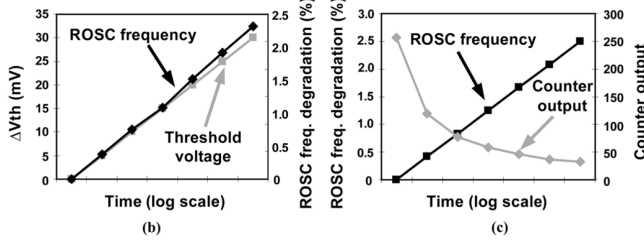
Fig. 4. Ring oscillator circuit and measurement/stress modes. (b) Simulation results of stress time versus pMOS threshold voltage and ring oscillator frequency. (c) Frequency and counter output as a function of stress time.
