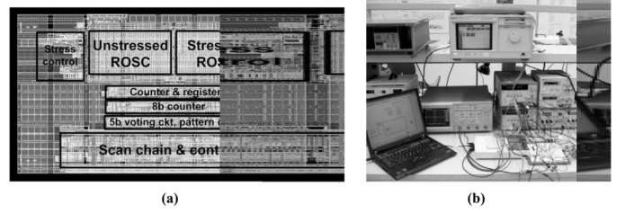
Fig. 7. (a) Layout of 130 nm test chip occupying 265 \times 132 \mu\text{m}^2 . (b) Laboratory setup for test chip NBTI measurements.
