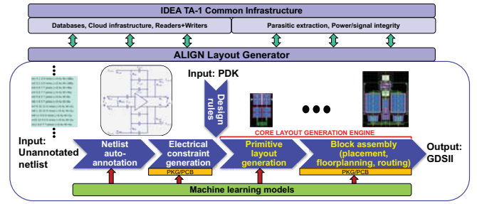
Figure 1: Overview of the ALIGN flow.
