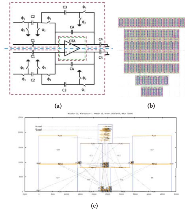
Figure 5: (a) A switched capacitor (SC) filter, and the ALIGN-generated layout of (b) the OTA within the SC filter and (c) the entire SC filter, where “CC” refers to a capacitor array. The opamp is placed on top; other transistors correspond to switches.
