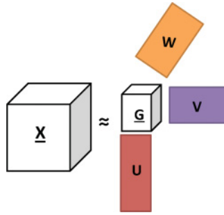
Fig. 2. The TUCKER3 decomposition of \underline{\mathbf{X}} .
