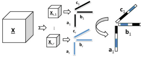
Fig. 4. Example of rank-1 PARAFAC using PARCUBE (Algorithm 3). The procedure described is as follows: create r independent samples of \mathbf{X} , using Algorithm 1. Run the PARAFAC-ALS algorithm for K = 1 and obtain r triplets of vectors, corresponding to the first component of \mathbf{X} . As a final step, combine those r triplets, by distributing their values to the original sized triplets, as indicated in Algorithm 3.
