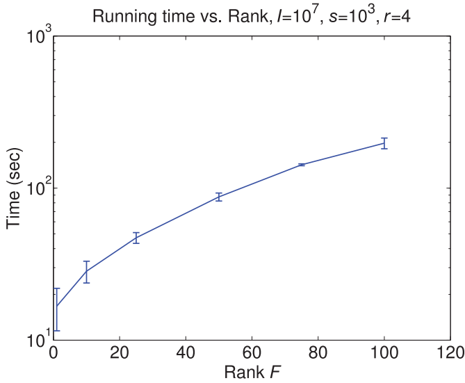
Fig. 12. Scalability with respect to the decomposition rank.
