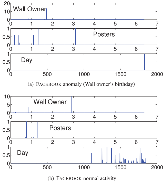
Fig. 17. Results for FACEBOOK using s = 100 , r = 10 , F = 15 . Subfigure (a): FACEBOOK “anomaly”: One Wall, many posters and only one day. This possibly indicates the birthday of the Wall owner. Subfigure (b): FACEBOOK “normal” activity: many users post on many users’ Walls, having a continuous daily activity
