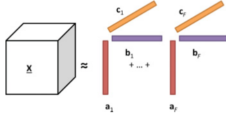
Fig. 1. The F -component PARAFAC decomposition of \underline{\mathbf{X}} .
