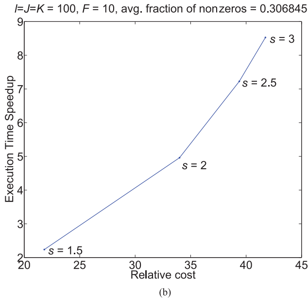
Fig. 5. PARCUBE is faster than ALS-PARAFAC: Speedup versus Relative cost (PARCUBE/ ALS-PARAFAC) for 1 repetition, for varying sampling factor and different degrees of sparsity. We observe that even for a relatively high sampling factor, we get relatively good relative cost, which may be further improved using repetition. Key here is that by using repetition, because this procedure may be carried out in parallel, we may improve the accuracy and maintain similar speedup.
