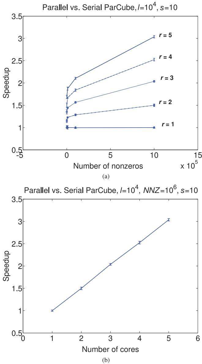
Fig. 9. Serial versus Parallel PARCUBE
