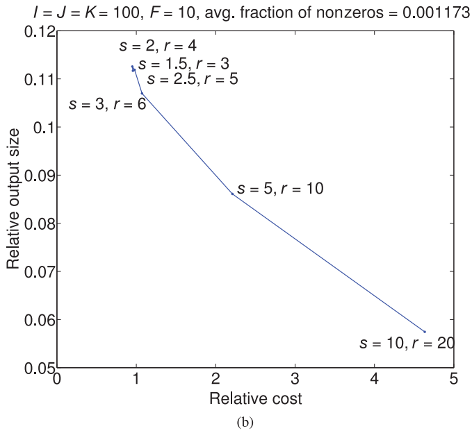
Fig. 7. PARCUBE outputs sparse factors: relative output size (PARCUBE/ ALS-PARAFAC) versus relative cost. We see that the results of PARCUBE are more than 90% sparser than the ones from Tensor Toolbox, while maintaining the same approximation error.
