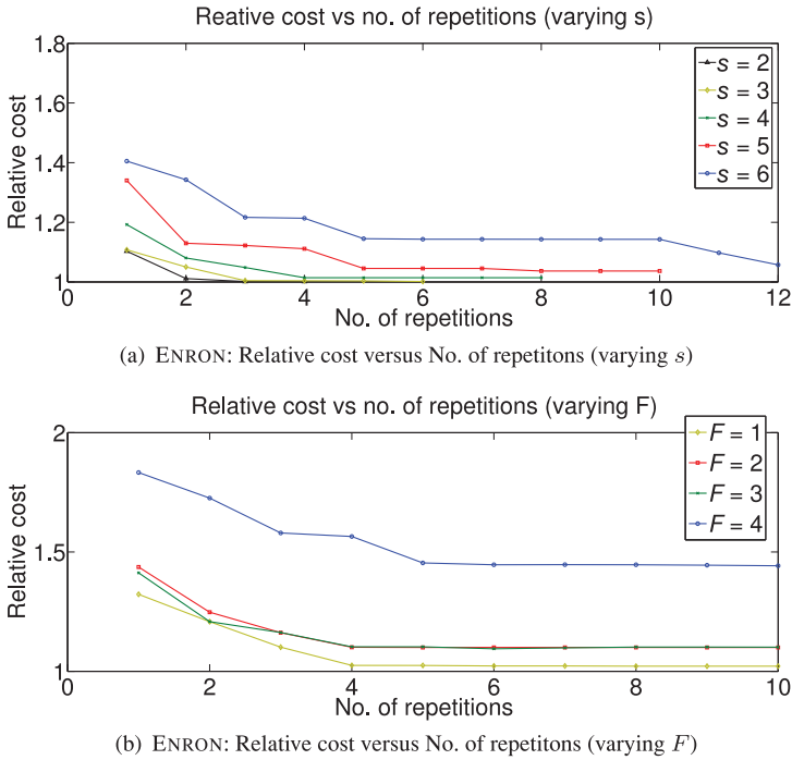
Fig. 6. PARCUBE reduces the PARAFAC approximation cost. (a) Approximation cost versus the number of repetitions for varying s , where r = 2s . (b) Approximation cost versus number of repetitions for varying F and fixed s = 5 . In both cases, the approximation improves as r increases, as expected.
