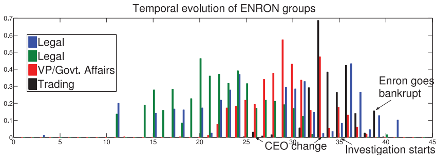
Fig. 15. Temporal evolution of four groups in the ENRON dataset. We have labelled the groups, according to the position of the participants in the company. The labels of the extracted groups are consistent with other works in the literature albeit they have been extracted with somewhat different order. We have also discovered two Legal groups that behave slightly differently over time, a fact probably stemming from the different people involved in each group.
