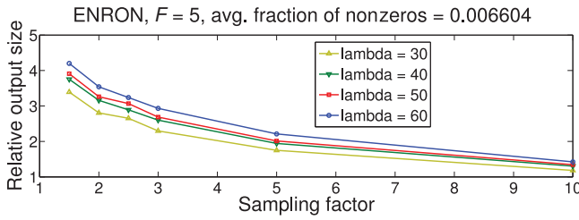
Fig. 8. PARCUBE outputs sparse factors: relative output size (PARCUBE/ PARAFAC SLF) versus sampling factor s (in which no. of repetitions is r = 2s ).
